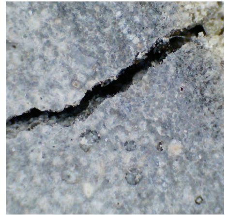
Concrete beam without AQUAFIX (0.5 mm crack)
